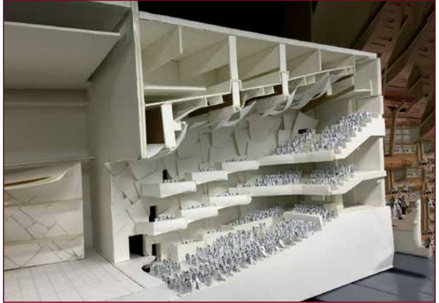
Builders made this styrofoam-and-paper model of the Musco Center for the Arts to test how sound would reflect off the ceiling, floor, wall “petals,” and audience.
